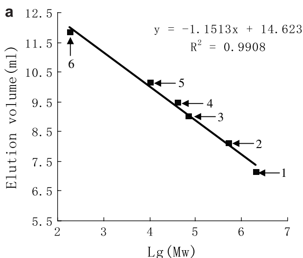
Fig. 1. Weight-average molecular weight determination by HPLC system of Agilent 1100 equipped with a gel-filtration chromatographic column of Shodex Sugar KS-805.
